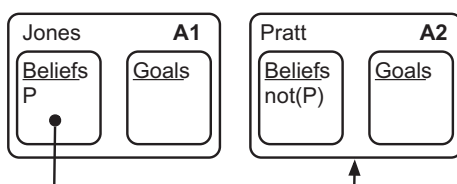
Fig. 1. False belief. A1 and A2 are agent models with separate belief and goal partitions. Here, Jones believes that Pratt falsely believes \text{not}(P) .
