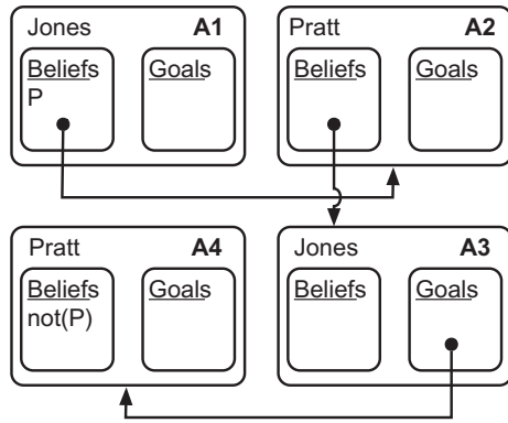
Fig. 3. Pandering. A1, A2, A3, and A4 are agent models. Here, Jones believes that Pratt's declaration of \text{not}(P) is pandering because Pratt thinks Jones wants Pratt to believe \text{not}(P) .
