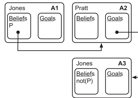
Fig. 2. Lying. A1, A2, and A3 are agent models. Here, Jones believes that Pratt has lied, wanting him to believe \text{not}(P) .
